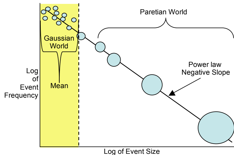
Figure 1 Stylized Pareto Distribution on Log-Log Scale
